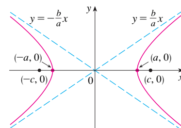
FIGURA 12 \frac{x^2}{a^2} - \frac{y^2}{b^2} = 1
