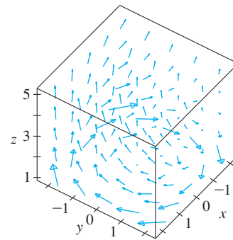
FIGURA 12 \mathbf{F}(x, y, z) = \frac{y}{z} \mathbf{i} - \frac{x}{z} \mathbf{j} + \frac{z}{4} \mathbf{k}
